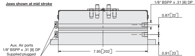
Jaws shown at mid stroke
