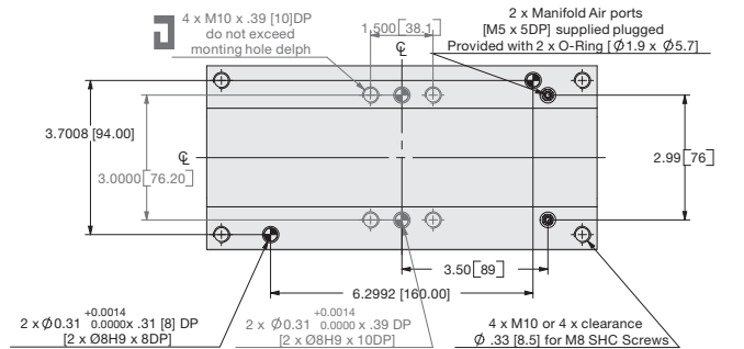
Jaws shown at mid stroke
